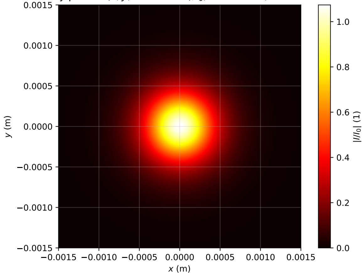
Intensity profile I(x, y, z = 3.105m)/I_0 , P_{in}=0.8P_{cr} , artificial time
